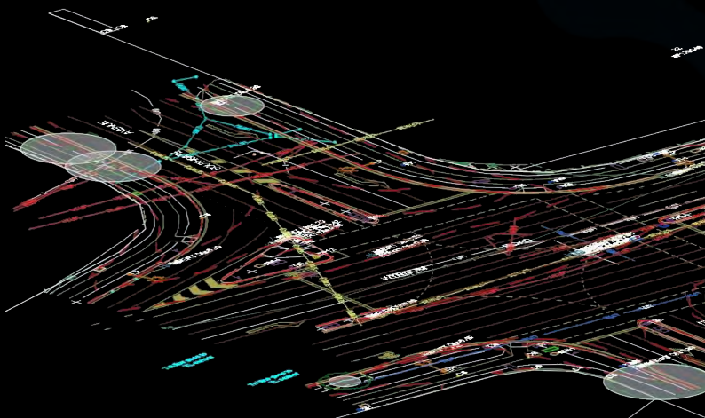
Surveyed subsurface utility data overlaid on topographic survey
